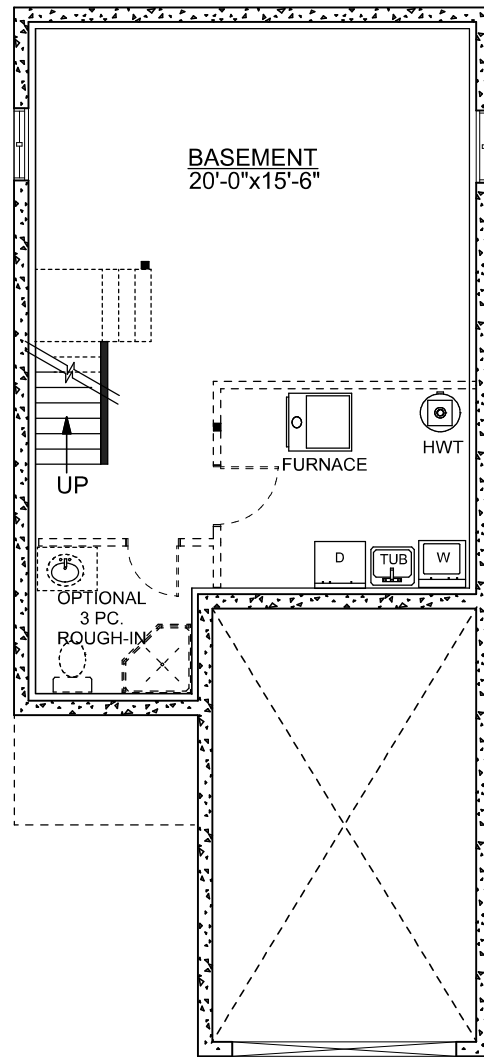
BASEMENT PLAN
