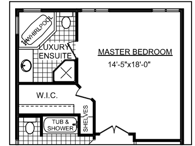
UPPER FLOOR WITH OPTIONAL LUXURY ENSUITE 5015-0011
