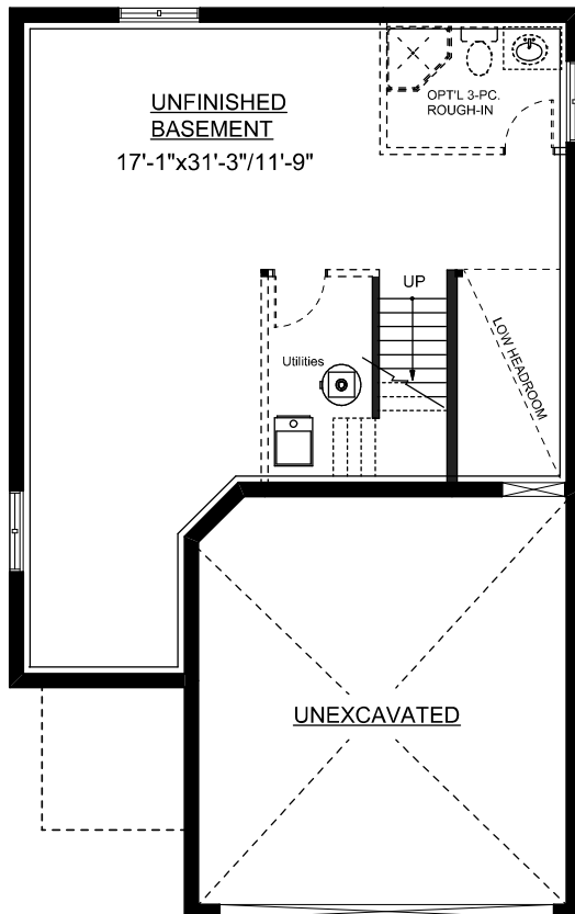
BASEMENT PLAN
