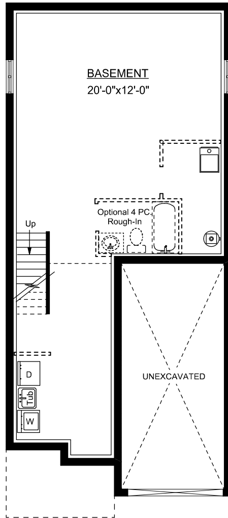
BASEMENT PLAN
